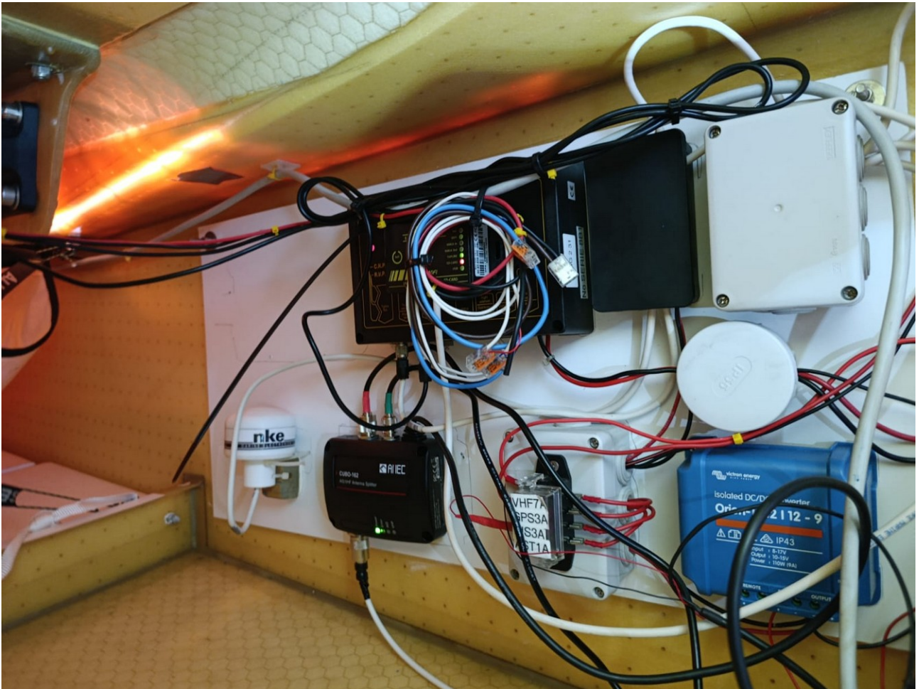
Solar panel regulators.
