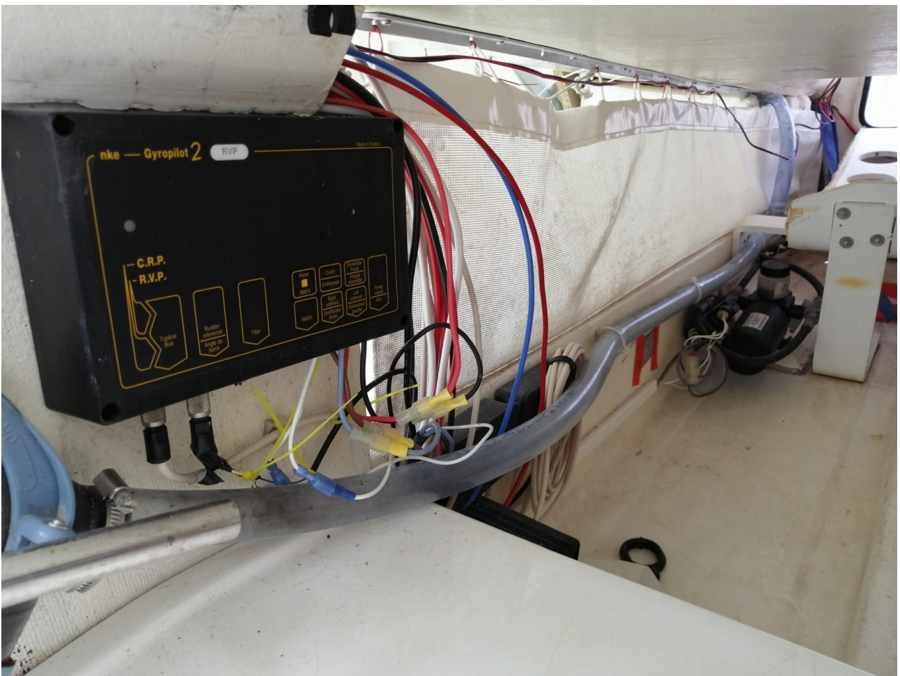
Gyropilot installation.
